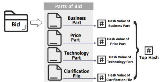
Figure 5. Top Hash
