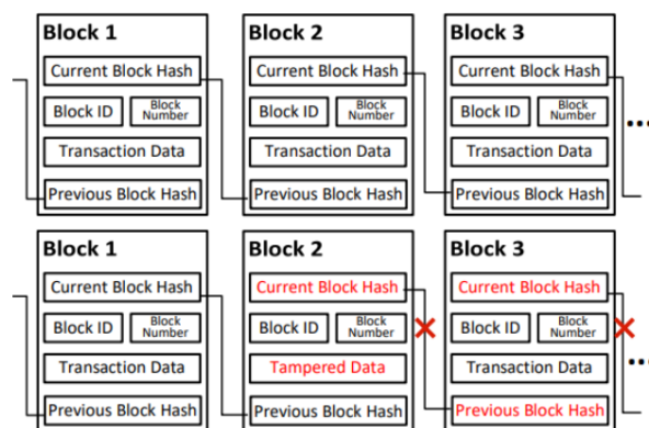
Figure 1. Blockchain Structure
