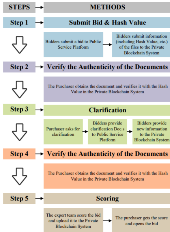
Figure 2. Framework Steps
