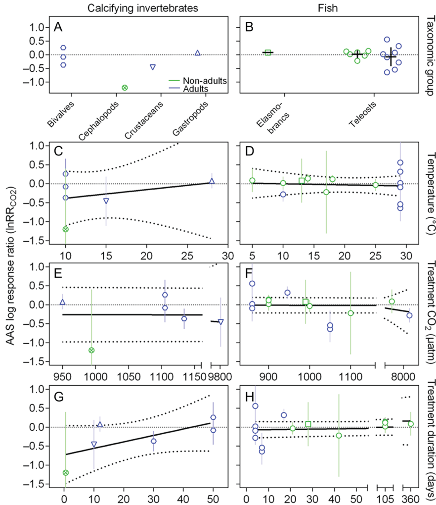
Figure 9: Effect of elevated CO 2 on absolute aerobic scope (AAS). Data are log response ratios to CO 2 (lnRR CO 2 ) of calcifying invertebrates ( A , C , E and G ) and teleosts and elasmobranchs ( B , D , F and H ) in non-adults (green) and adults (blue) of different taxonomic groups (inverted triangle, crustacean; upright triangle, gastropod; hexagon, bivalve; circled cross, cephalopod; square, elasmobranch; and circle, teleost). Data are also depicted as a function of the temperature at which the experiment was conducted (C and D), as a function of the PCO 2 used as the experimental treatment (E and F) and as a function of the duration of the CO 2 exposure (G and H). Note that the invertebrate species are all calcifying because there were no comparable data available for non-calcifying species. Continuous lines indicate mean ± 95% confidence interval (A and B) or fitted lines from linear regression, with dotted lines representing the 95% confidence interval (C–H) (see Results for details). The complete data set and reference details are available in Supplementary Table ST2_AAS .
