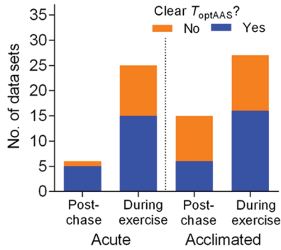
Figure 6: Effect of methodology on the presence or absence of an optimal temperature for absolute aerobic scope ( T_{optAAS} ). Data are the number of data sets with absence or presence of a T_{optAAS} ('no' or 'yes') grouped by methodology ('acute' or 'acclimated', and 'post-chase' or 'exercise'). There was no significant difference in the proportion of 'yes' and 'no' outcomes between the two methods in either acute or acclimated studies (see Results for details).
