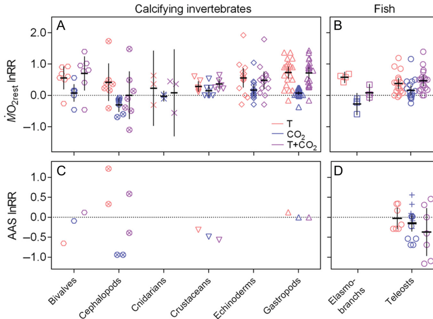
Figure 7: Isolated and combined effects of elevated temperature and partial pressure of CO 2 ( PCO_2 ) on resting oxygen uptake ( MO_{2rest} ) and absolute aerobic scope (AAS). Data are log response ratios ( \lnRR ) of MO_{2rest} (A and B) and AAS (C and D) in marine invertebrates (A and C) and fish (B and D) to elevated temperature alone (red symbols), elevated PCO_2 alone (blue symbols) and the combined treatment (purple symbols). Different shapes indicate different taxonomic groups (upright triangle, gastropod; circled cross, cephalopod; hexagon, bivalve; inverted triangle, crustacean; diamond, echinoderm; cross, cnidarian; square, elasmobranch; and circle, teleost). Note that the invertebrate species are all calcifying because there were no comparable data available for non-calcifying species. Continuous lines indicate mean \pm 95% confidence intervals. In (D), \lnRR from studies investigating CO 2 only (indicated by plus signs) have been added to illustrate the variation in responses, because this is not reflected in the studies having investigated both temperature and CO 2 . The complete data set and reference details are available in Supplementary Table ST3_MO2rest and ST3_AAS .
