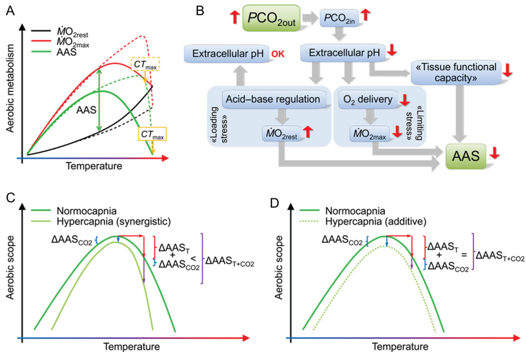
Figure 1: Proposed effects of temperature and CO 2 on aerobic performance. (A) The Fry paradigm (continuous lines), where resting oxygen uptake ( \dot{M}O_{2\text{rest}} ) is predicted to increase exponentially with temperature, whereas maximal oxygen uptake ( \dot{M}O_{2\text{max}} ) reaches an optimum and then declines. As a result, the absolute aerobic scope (AAS = \dot{M}O_{2\text{max}} - \dot{M}O_{2\text{rest}} ) is represented by a bell-shaped curve, and the optimum for AAS ( T_{\text{optAAS}} ) is assumed to reflect the overall optimum for fitness ( T_{\text{optFIT}} ). Alternatively (dashed lines), it can be proposed that the increase in \dot{M}O_{2\text{rest}} may be less pronounced, because of acclimation, and that \dot{M}O_{2\text{max}} is not limited to the same degree at higher temperature (Clark et al. , 2013; Schulte, 2015), resulting in a scope that continues to increase until the critical temperature CT_{\text{max}} (that is, where the animal eventually will die). In this case, it is unlikely that T_{\text{optAAS}} coincides with T_{\text{optFIT}} . (B) Elevated CO 2 in the water ( PCO_{2\text{out}} ) has been proposed by some authors to cause a reduction in aerobic scope through ‘reduced tissue functional capacity’ (Pörtner, 2012) or by causing an elevation in \dot{M}O_{2\text{rest}} (loading stress) and/or a decrease in \dot{M}O_{2\text{max}} (limiting stress; Heuer and Grosell, 2014). (C) Change in the aerobic scope curve if simultaneous exposure to elevated temperature and hypercapnia has a synergistic effect, where the isolated effect of CO 2 ( \Delta AAS_{CO_2} ) at the thermal optimum is small, or zero, but exacerbated when temperature rises, causing further reduction in aerobic scope (e.g. Pörtner et al. , 2005). The combined effect ( \Delta AAS_{T+CO_2} ) is thus larger than expected from the sum of the two isolated effects ( \Delta AAS_T and \Delta AAS_{CO_2} ). (D) Alternatively, hypercapnia can cause a reduction in AAS ( \Delta AAS_{CO_2} ) independent of temperature, and the combined effect of the two stressors is then additive.
