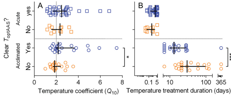
Figure 4: Effect of temperature coefficient ( Q_{10} ) and acclimation time on the presence (yes) or absence (no) of an optimal temperature ( T_{optAAS} ) for absolute aerobic scope. (A) Presence or absence of T_{optAAS} as a function of Q_{10} for resting oxygen uptake. (B) Presence or absence of T_{optAAS} as a function of the duration of temperature treatment in studies using acute treatment and acclimation. Continuous lines indicate median \pm interquartile range. Note the logarithmic scale in (B). Asterisk indicates significant difference in Q_{10} and acclimation duration, in studies with different outcome for acclimated species (* P < 0.05 , *** P < 0.001 ; see 'Results' for details).
