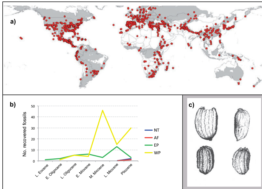
FIGURE 1. a) Potential distribution of Hypericum in the present (in grey); the map was created by projecting the climatic tolerances of extant Hypericum species based on 1033 occurrences (red dots) over present climatic conditions. b) Number of fossil remains of Hypericum through time and across biogeographic regions. Line colors correspond with the discrete areas defined in the inset map of Figure 4. c) Fossil seeds of Hypericum antiquum Balueva & Nikitin, 4 seeds, \times 33 (reproduced with permission from Arbuzova 2005). Color version of this figure is available at Systematic Biology online.
