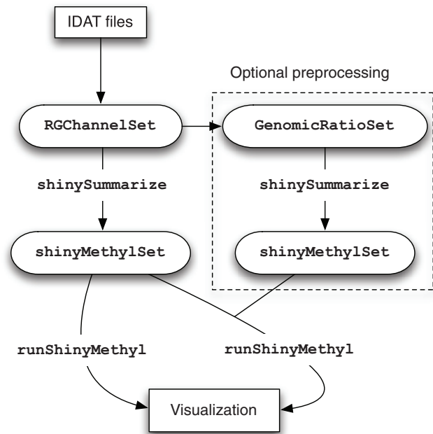
Figure 1. The workflow of shinyMethyl . IDAT files are parsed using minfi and illuminaio into a RGChannelSet . This object is summarized using shinySummarize . Optionally, the data are pre-processed and the pre-processed data are summarized. For visualization, runShinyMethyl is used on either one or two sets of summarized data.
