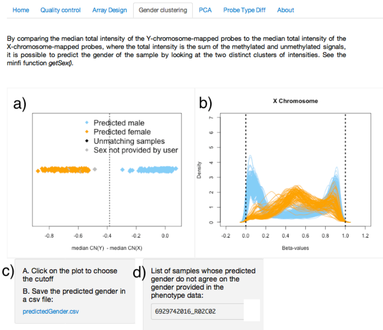
Figure 4. Sex prediction interface. The difference of the median copy number intensity for the Y chromosome and the median copy number intensity for the X chromosome can be used to separate males and females. In a) , the user can select the vertical cutoff (dashed line) manually with the mouse to separate the two clusters (orange for females, blue for males). Corresponding Beta-value densities appear in b) for further validation. The predicted sex can be downloaded in a csv file in c) , and samples for which the predicted sex differs from the sex provided in the phenotype will appear in d) .
