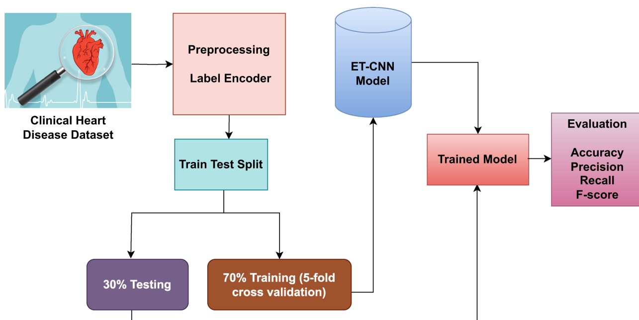
Figure 4. Workflow diagram of the proposed model.
