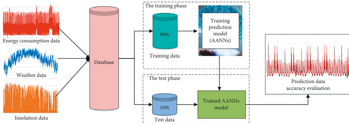
FIGURE 4: Implementation of the AANNs model.
